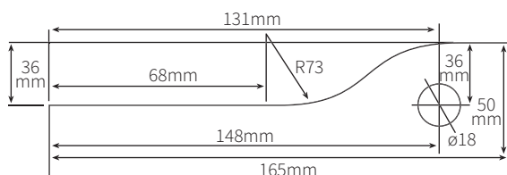
GLASS CUT OUT DETAIL
