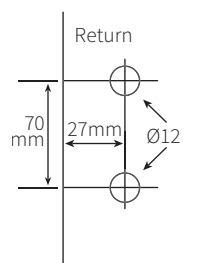
GLASS CUT OUT DETAIL
