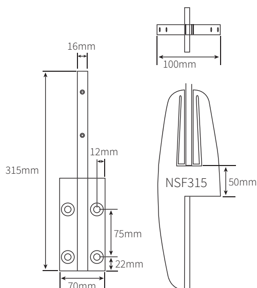
FIXING DETAIL - DOMESTIC WOOD FIX (CSW100)
