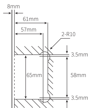
GLASS CUT OUT TOP AND BOTTOM
