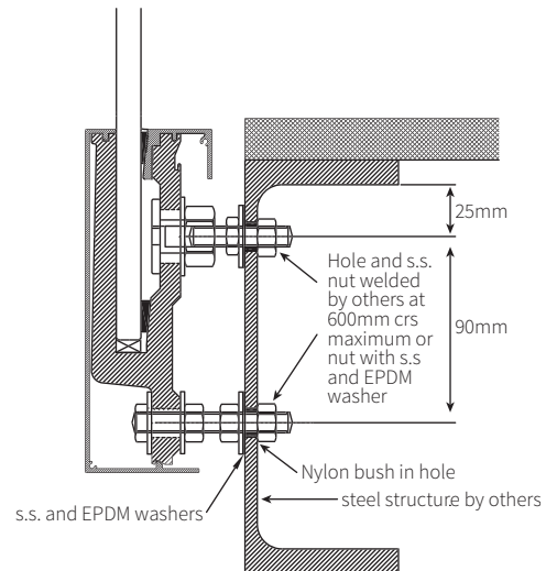
FIXING DETAIL - STEEL (EXTERNAL & INTERNAL)
