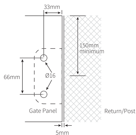
GLASS CUT OUT DETAIL
