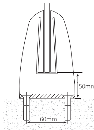
FIXING DETAIL - DOMESTIC CONCRETE FIX (MF43)
