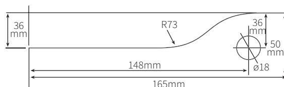
GLASS CUT OUT DETAIL
