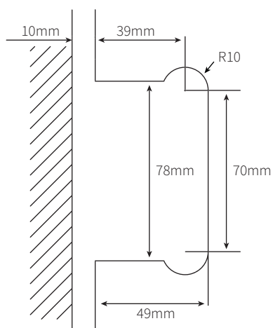
GLASS CUT OUT DETAIL - WALL TO GLASS
