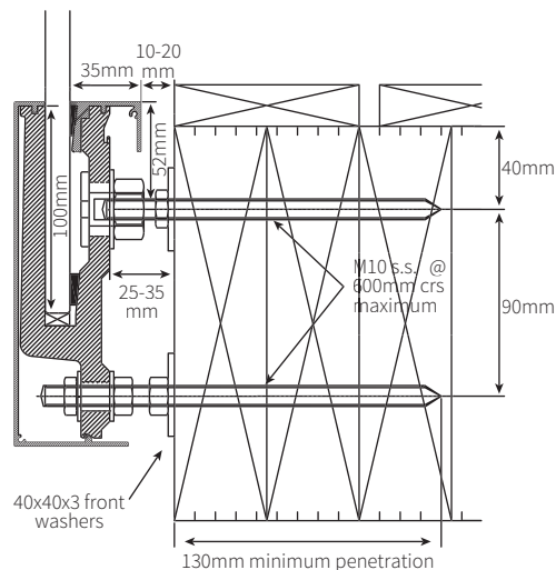
FIXING DETAIL - TIMBER SLATTED DECK LAG SCREW FIXING
