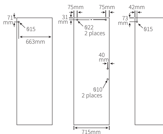
Side panel 10mm glass thickness
