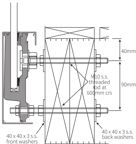
FIXING DETAIL - TIMBER SLATTED DECK BOLT THROUGH FIXING
