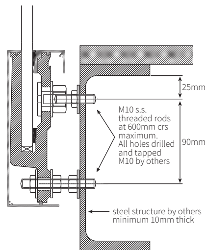
FIXING DETAIL - STEEL (INTERNAL)
