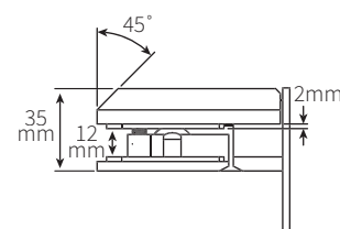
BASE VIEW
