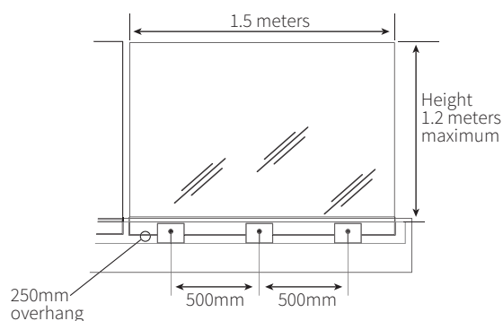
Residential A, C3 and Pool Fence
