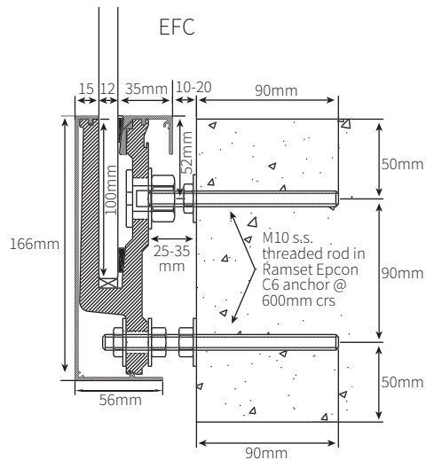
FIXING DETAIL - CONCRETE
