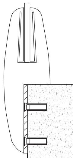
FIXING DETAIL - DOMESTIC CONCRETE FIX (MF43)
