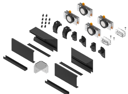
SV-X50 kit angular 90° - KIT 2 x2 Retaining stopper
