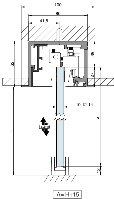
TRACK 3 Wall / Ceiling mount with fixed panel
