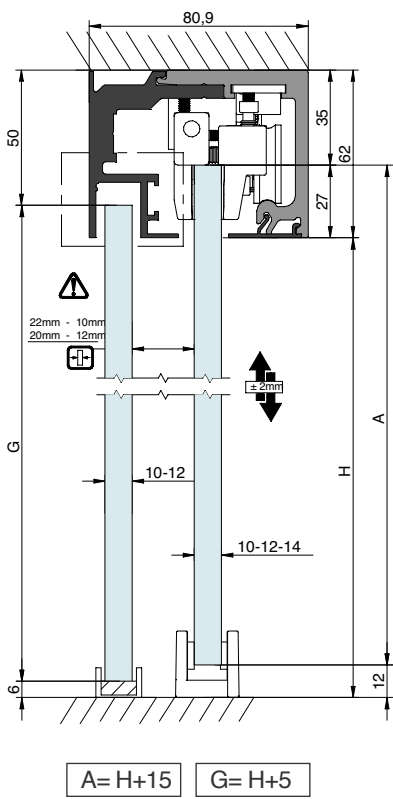
TRACK 3 Wall / Ceiling mount with fixed panel
