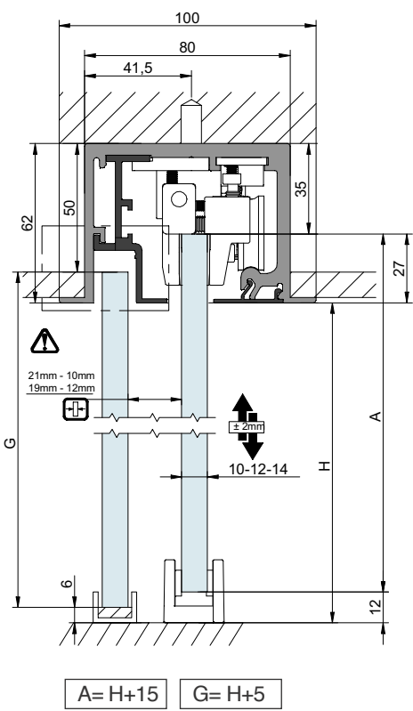
TRACK 4 False ceiling mount with fixed panel
