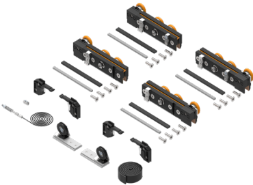
SV-Sincro Q110 Fitting set x2 Retaining stopper
