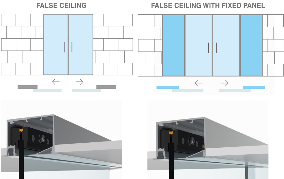
CUBE PELMET COVER
